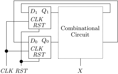
Figure 2: Sequential circuit 図 2 : 順序回路
